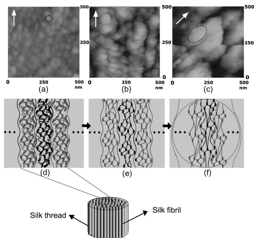
FIGURE 7 Topographic AFM image of spider dragline silk N. pilipes at different reeling speeds and the proposed model for the corresponding structure change with increasing reeling speed: (a) at 2.5 mms ^{-1} , (b) at 25 mms ^{-1} , and (c) at 100 mms ^{-1} . The direction of thread is indicated by the arrow. (d) At low reeling speed ( <2 mms ^{-1} ), crystallites are less well-oriented and the amorphous chains are relaxed. (e) With increasing reeling speed, the crystallites are smaller and better oriented. At the same time, the intercrystallite distance becomes larger. (f) Further increase of the reeling speed ( >10 mms ^{-1} ) causes nanofibrils to merge further together, and the observed “particle size” as indicated by a dashed circle becomes larger, thus the distance between the crystallites becomes smaller.
