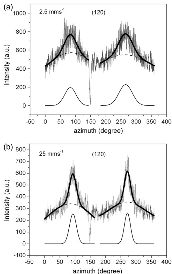
FIGURE 3 Intensity as a function of azimuth angle at the radial position of the equatorial (120) peak: (a) at 2.5 mm s -1 and (b) at 25 mm s -1 . The peaks are fitted as sums of two Gaussians, corresponding to crystalline (narrow) and amorphous (broad) distributions.
