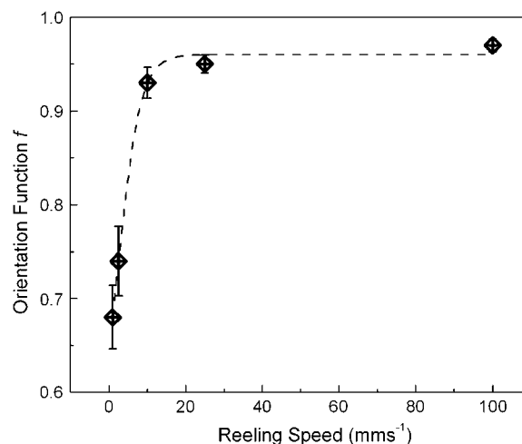
FIGURE 4 Orientation function f , calculated from FWHM, increases with reeling speed.
